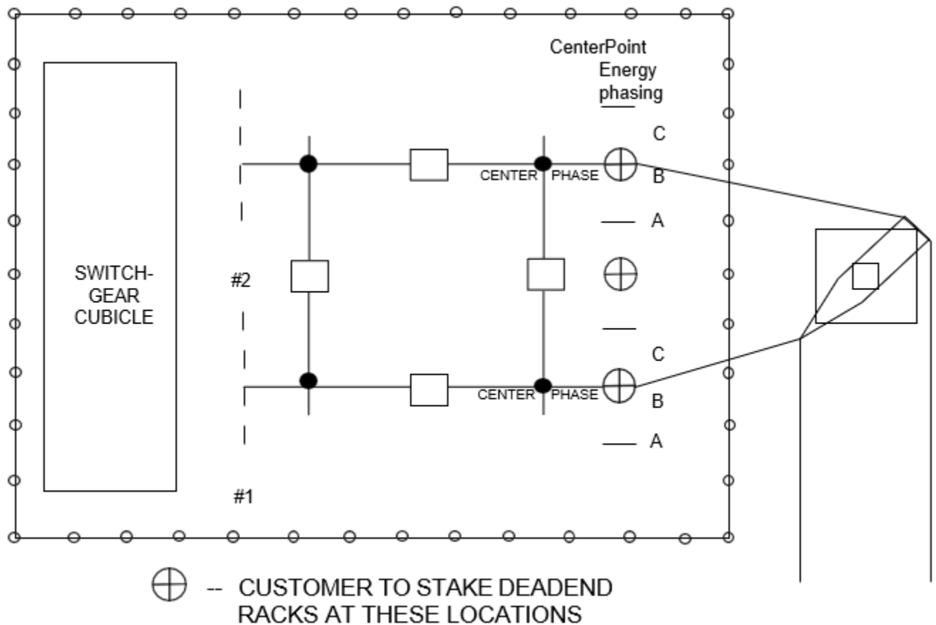
Figure 4 Staking Requirements for Typical Customer Substation
