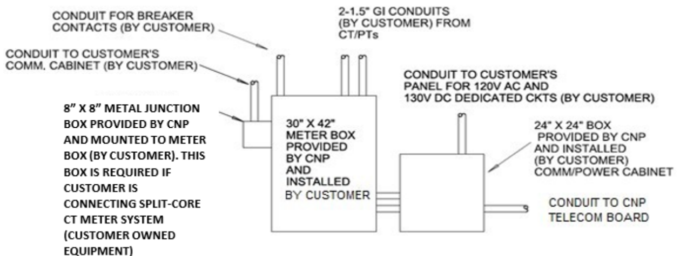
Figure 5 Typical Layout of Meter Boxes
