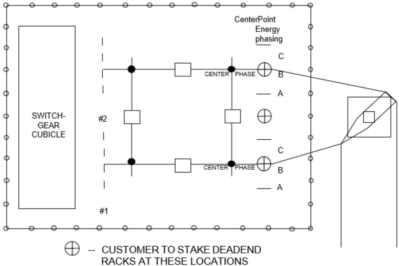
Figure 8 Staking Requirements for Typical Customer Substation
