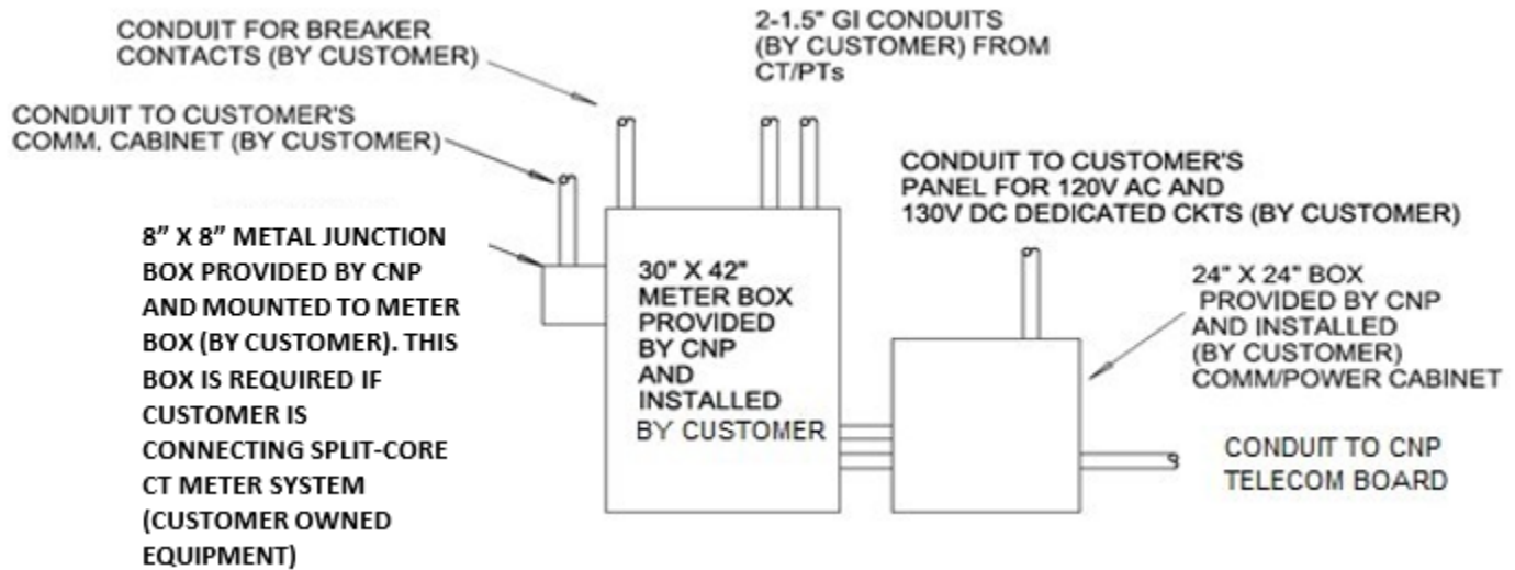
Figure 9 Typical Layout of Meter Boxes
