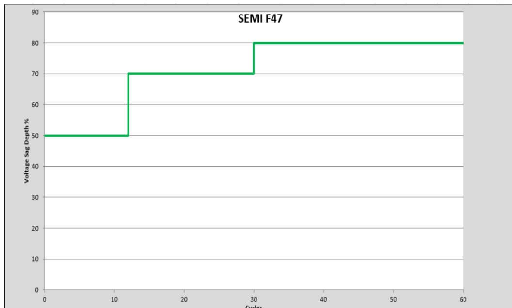
Figure 1 SEMI-F47 Voltage Ride Through design criteria
